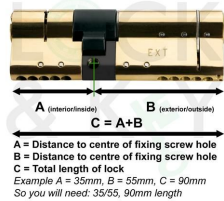
How to measure ABS cylinder lock:
